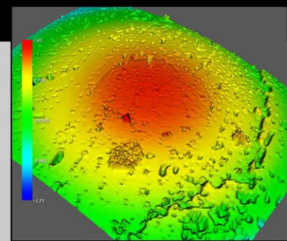
Interferometer image of 3D debris and contamination (courtesy of FIBO)
